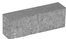
Dito 8 240 × 60 × 80 mm
